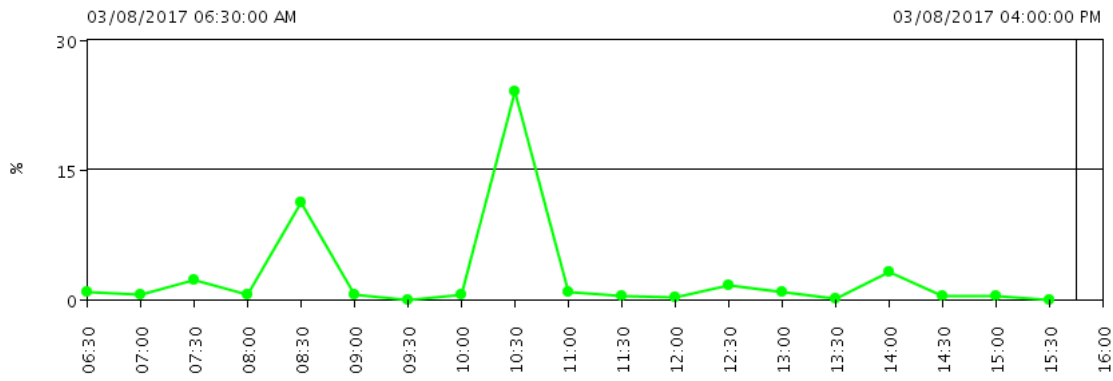
VMStat : User CPU Usage
